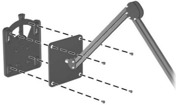
Figure 3-16 Installing the Quick Release
